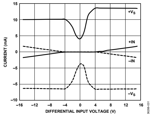
Figure 29. Fault Current Draw vs. Input Voltage, G = 10 , R_L = 10\text{ k}\Omega
