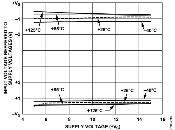
Figure 28. Input Voltage Limit vs. Supply Voltage, G = 1 , V_{REF} = 0\text{ V} , R_L = 10\text{ k}\Omega
