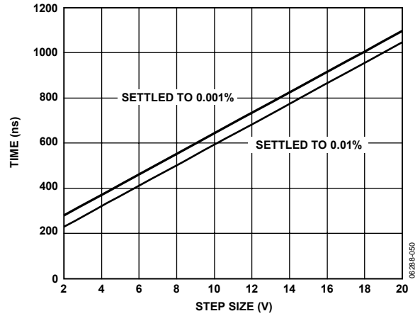
Figure 45. Settling Time vs. Step Size, G = 5 , R_L = 10\text{ k}\Omega
