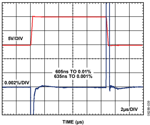
Figure 37. Large Signal Pulse Response and Settling Time G = 5, R_L = 10\text{ k}\Omega
