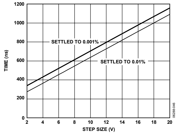
Figure 46. Settling Time vs. Step Size, G = 10 , R_L = 10\text{ k}\Omega
