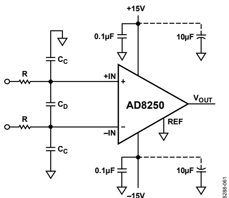
Figure 54. RFI Suppression
