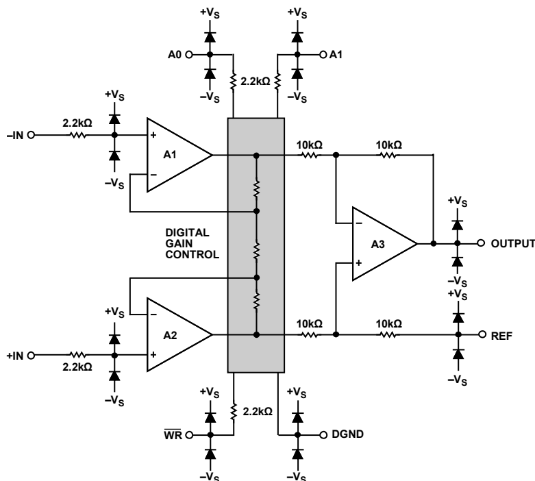
Figure 47. Simplified Schematic
