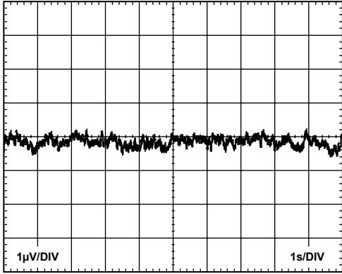
Figure 12. 0.1 Hz to 10 Hz RTI Voltage Noise, G = 10
